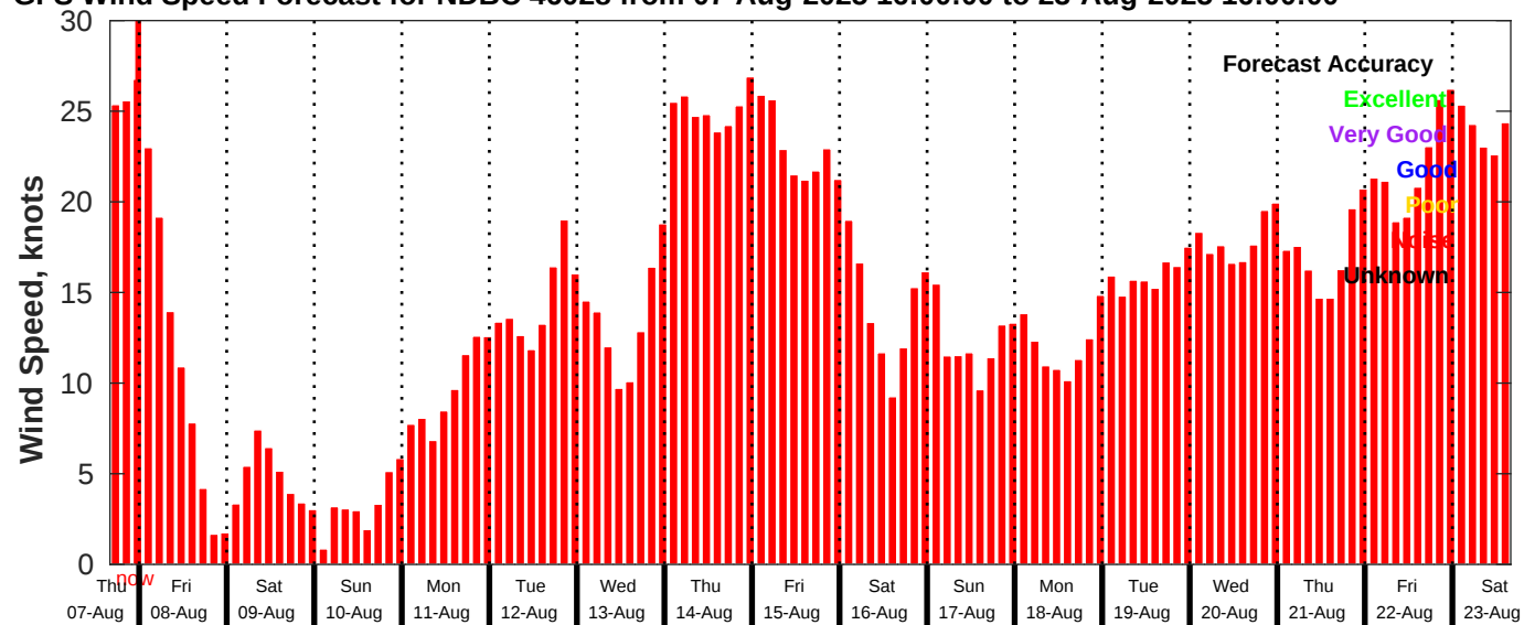
GFS Wind Speed Forecast for NDBC 46028 from 07-Aug-2025 16:00:00 to 23-Aug-2025 16:00:00
