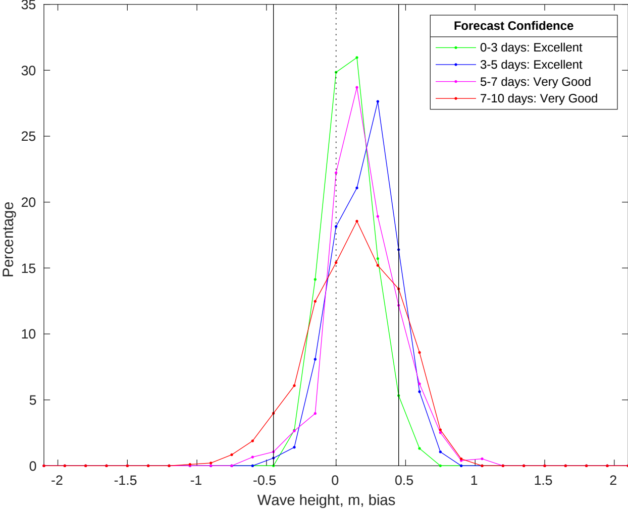
NDBC 46054 vs CMEMS Waves Bias Histogram: 08-Aug-2025
