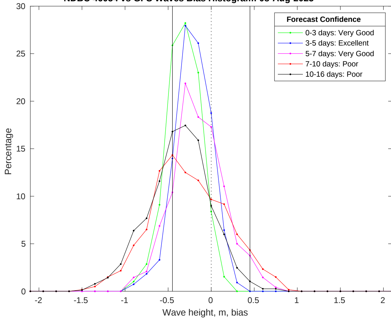
NDBC 46054 vs GFS Waves Bias Histogram: 08-Aug-2025
