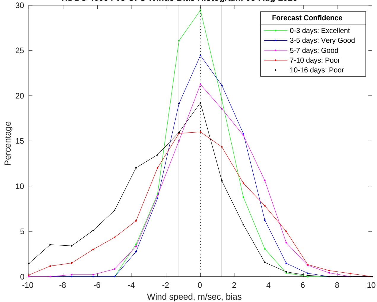
NDBC 46054 vs GFS Winds Bias Histogram: 08-Aug-2025
