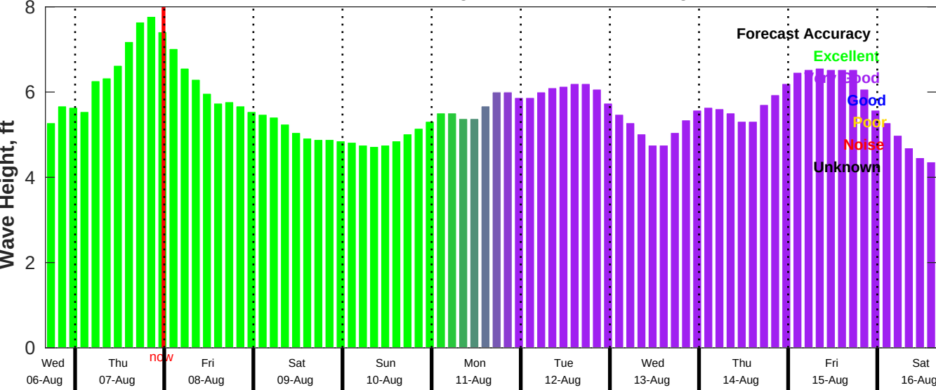
CMEMS Wave Forecast for NDBC 46054 from 06-Aug-2025 16:00:00 to 16-Aug-2025 16:00:00
