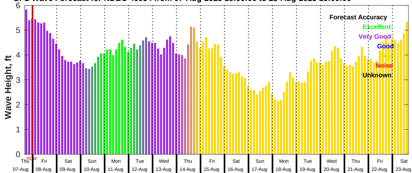
GFS Wave Forecast for NDBC 46054 from 07-Aug-2025 16:00:00 to 23-Aug-2025 16:00:00
