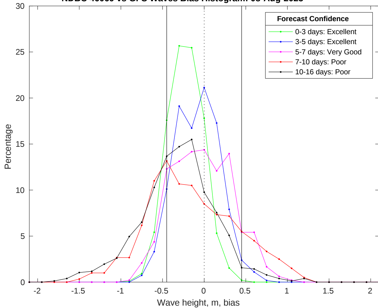
NDBC 46069 vs GFS Waves Bias Histogram: 08-Aug-2025
