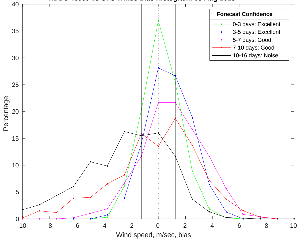
NDBC 46069 vs GFS Winds Bias Histogram: 08-Aug-2025
