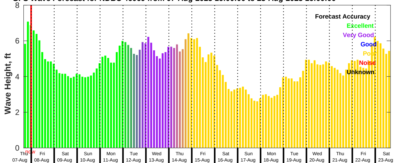
GFS Wave Forecast for NDBC 46069 from 07-Aug-2025 16:00:00 to 23-Aug-2025 16:00:00
