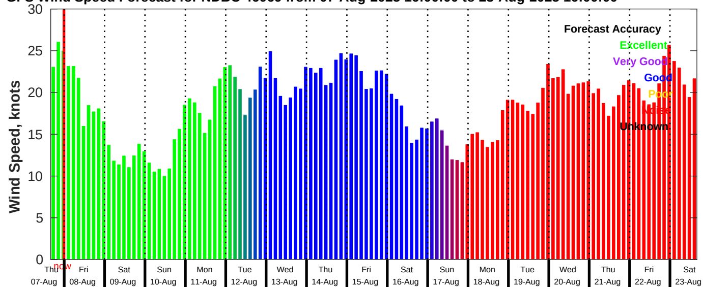
GFS Wind Speed Forecast for NDBC 46069 from 07-Aug-2025 16:00:00 to 23-Aug-2025 16:00:00
