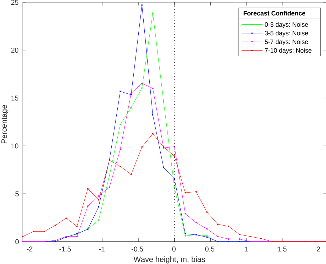
NDBC 51209 vs CMEMS Waves Bias Histogram: 08-Aug-2025
