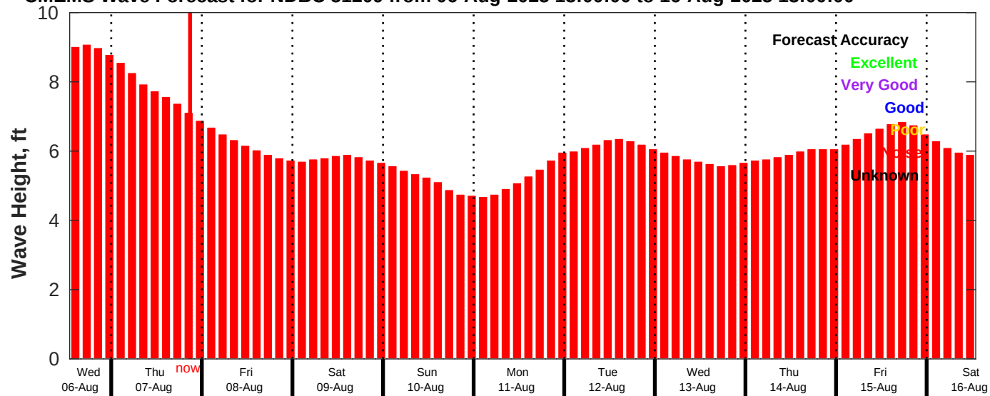
CMEMS Wave Forecast for NDBC 51209 from 06-Aug-2025 13:00:00 to 16-Aug-2025 13:00:00
