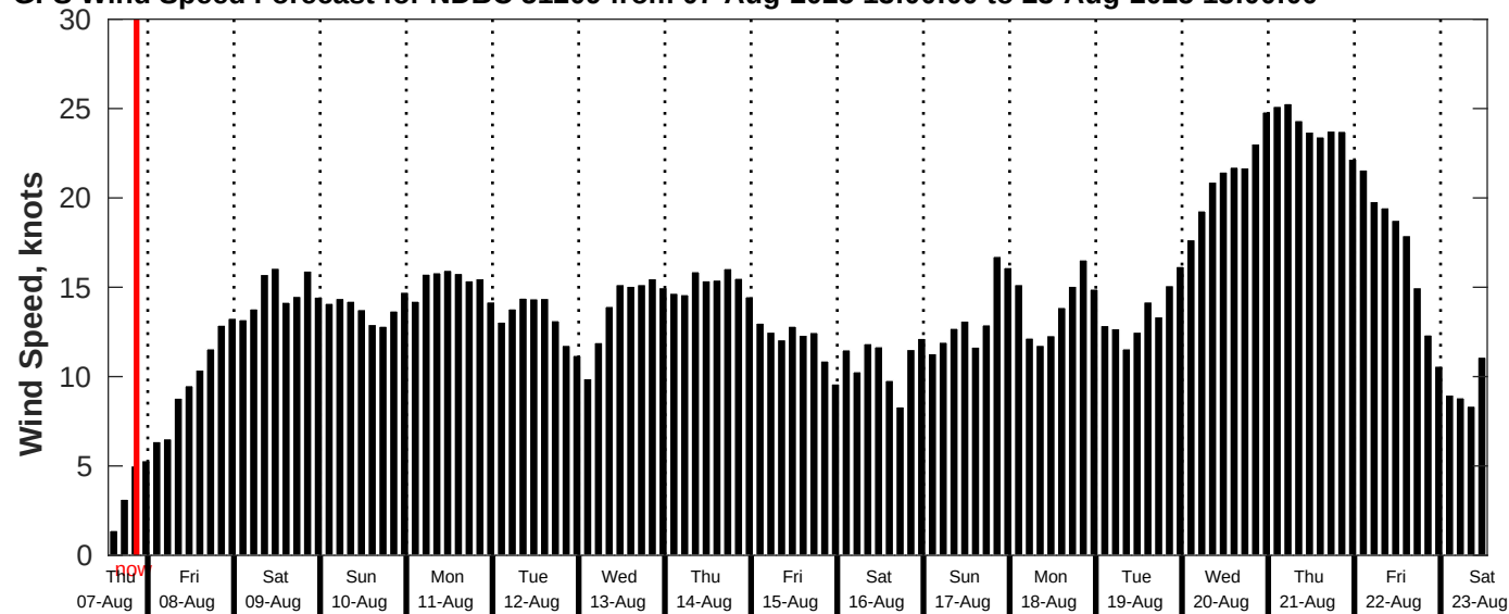
GFS Wind Speed Forecast for NDBC 51209 from 07-Aug-2025 13:00:00 to 23-Aug-2025 13:00:00
