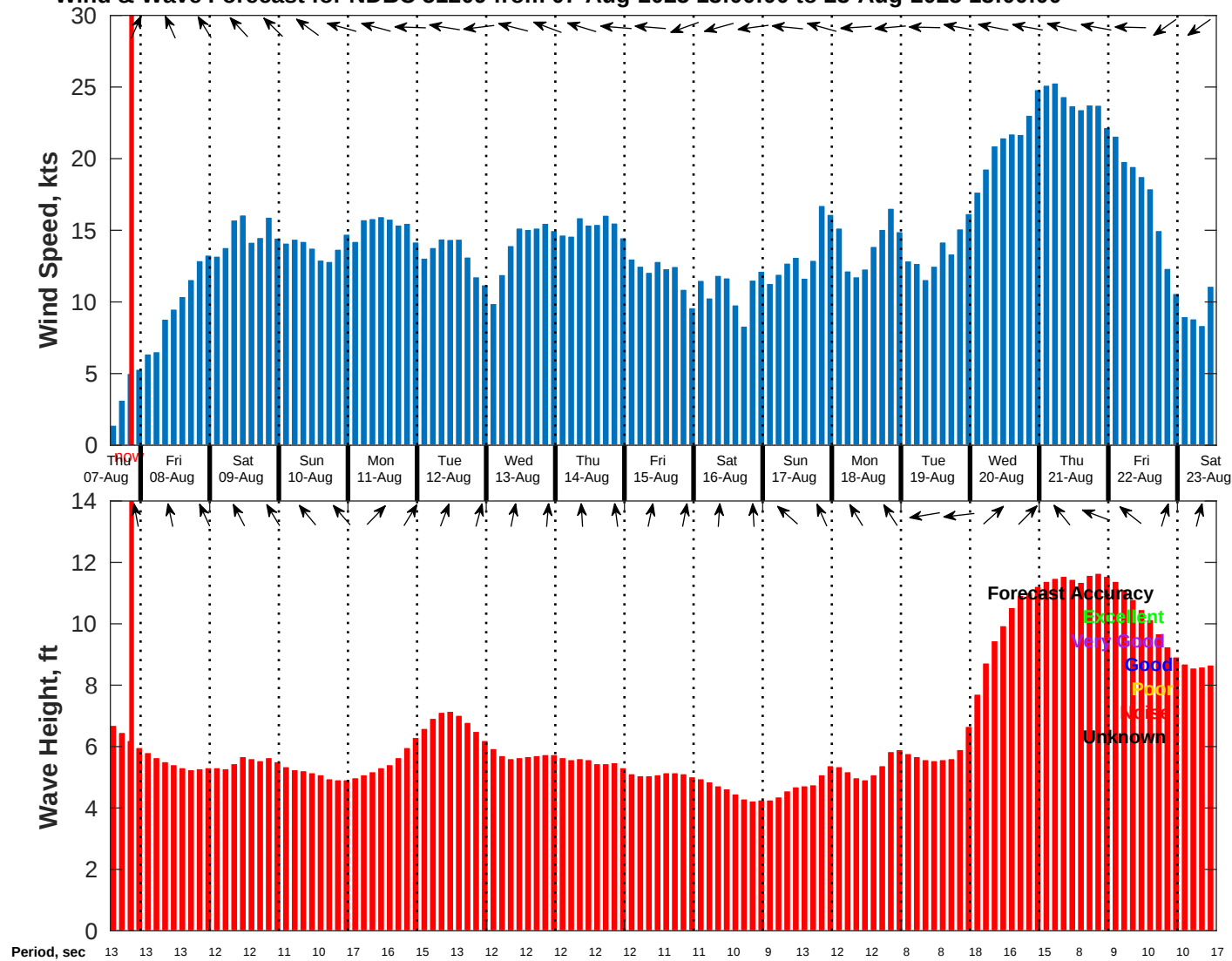
Wind & Wave Forecast for NDBC 51209 from 07-Aug-2025 13:00:00 to 23-Aug-2025 13:00:00
