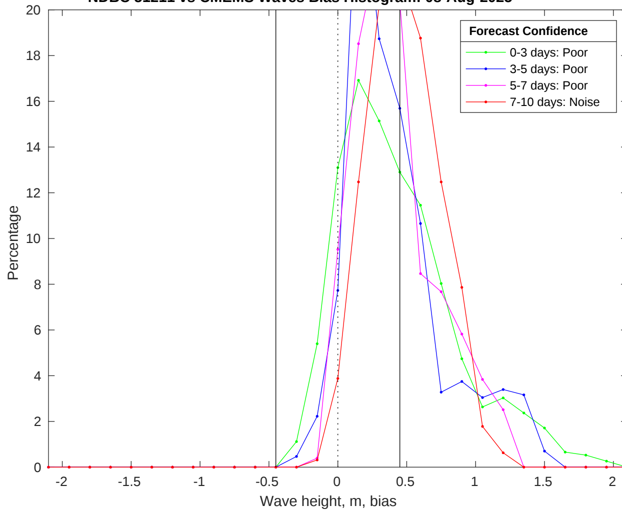
NDBC 51211 vs CMEMS Waves Bias Histogram: 08-Aug-2025
