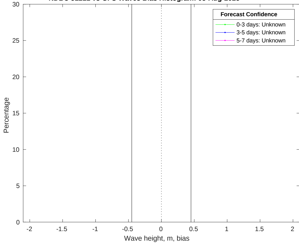
NDBC 51211 vs GFS Waves Bias Histogram: 08-Aug-2025
