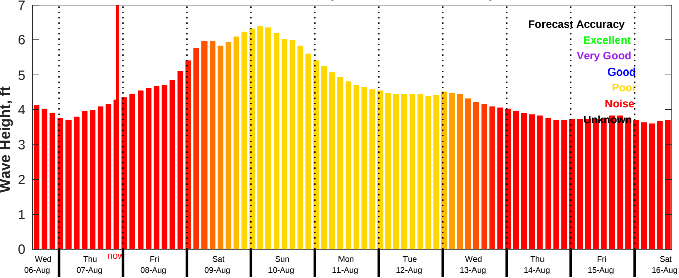
CMEMS Wave Forecast for NDBC 51211 from 06-Aug-2025 14:00:00 to 16-Aug-2025 14:00:00
