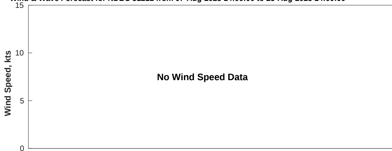
Wind & Wave Forecast for NDBC 51211 from 07-Aug-2025 14:00:00 to 23-Aug-2025 14:00:00
