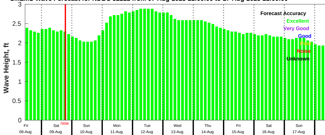
CMEMS Wave Forecast for NDBC 52211 from 07-Aug-2025 11:00:00 to 17-Aug-2025 11:00:00
