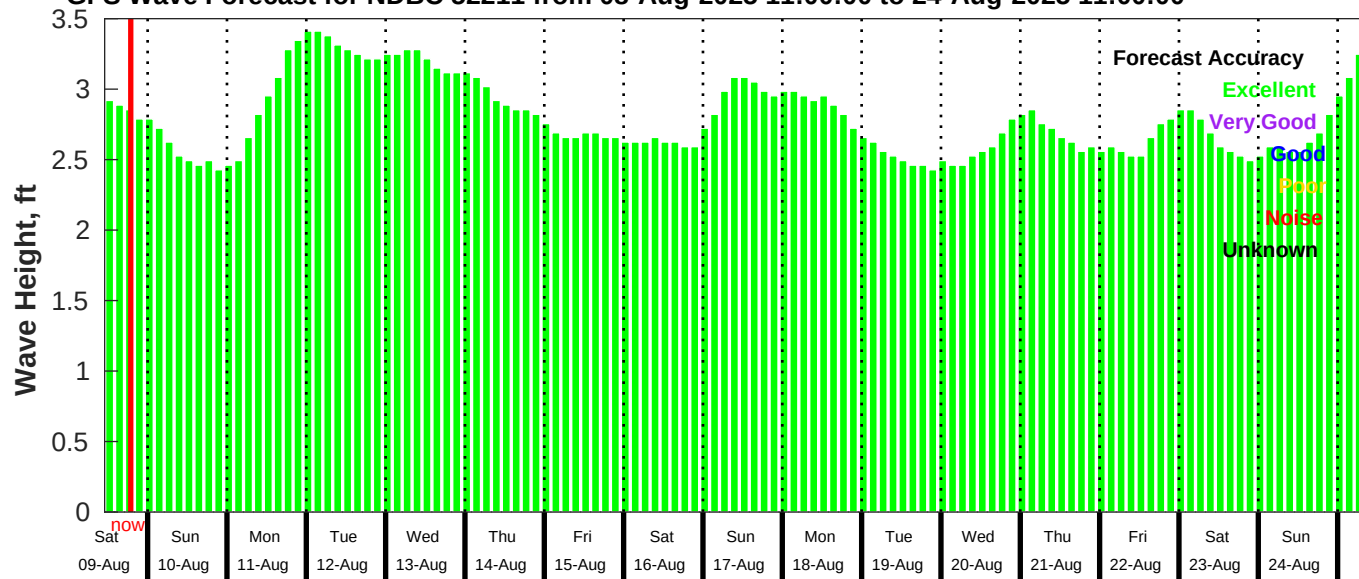
GFS Wave Forecast for NDBC 52211 from 08-Aug-2025 11:00:00 to 24-Aug-2025 11:00:00
