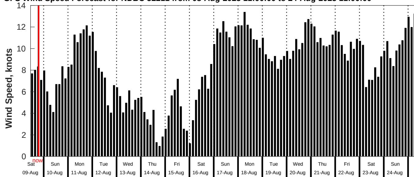
GFS Wind Speed Forecast for NDBC 52211 from 08-Aug-2025 11:00:00 to 24-Aug-2025 11:00:00
