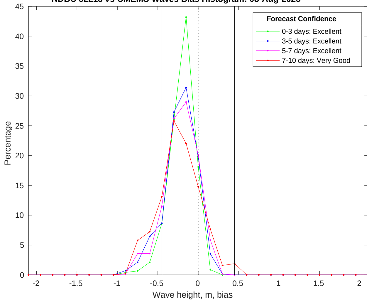
NDBC 52213 vs CMEMS Waves Bias Histogram: 08-Aug-2025
