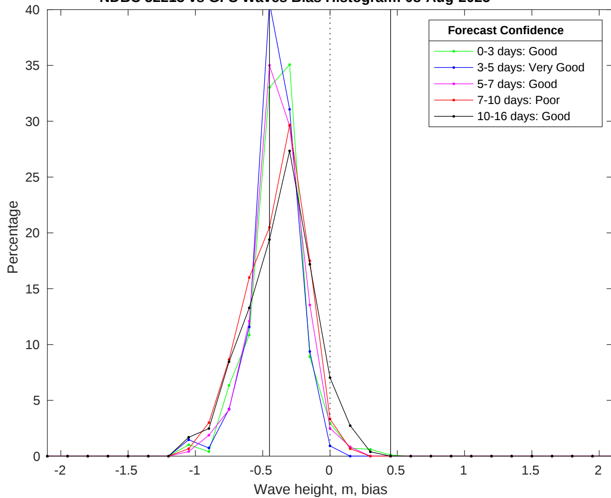
NDBC 52213 vs GFS Waves Bias Histogram: 08-Aug-2025
