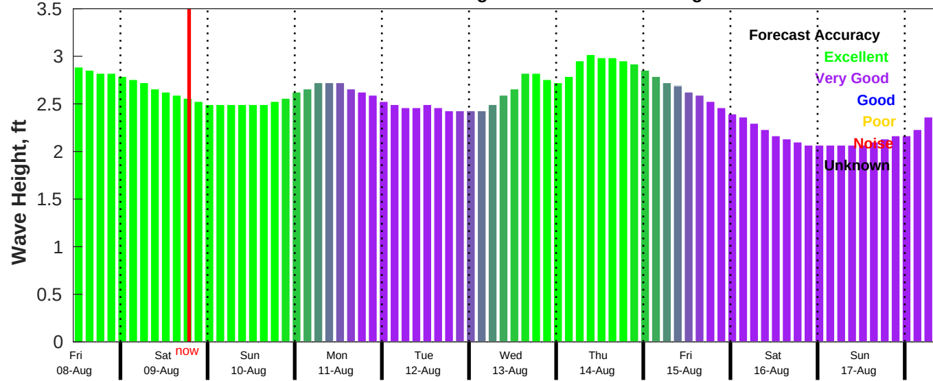
CMEMS Wave Forecast for NDBC 52213 from 07-Aug-2025 11:00:00 to 17-Aug-2025 11:00:00
