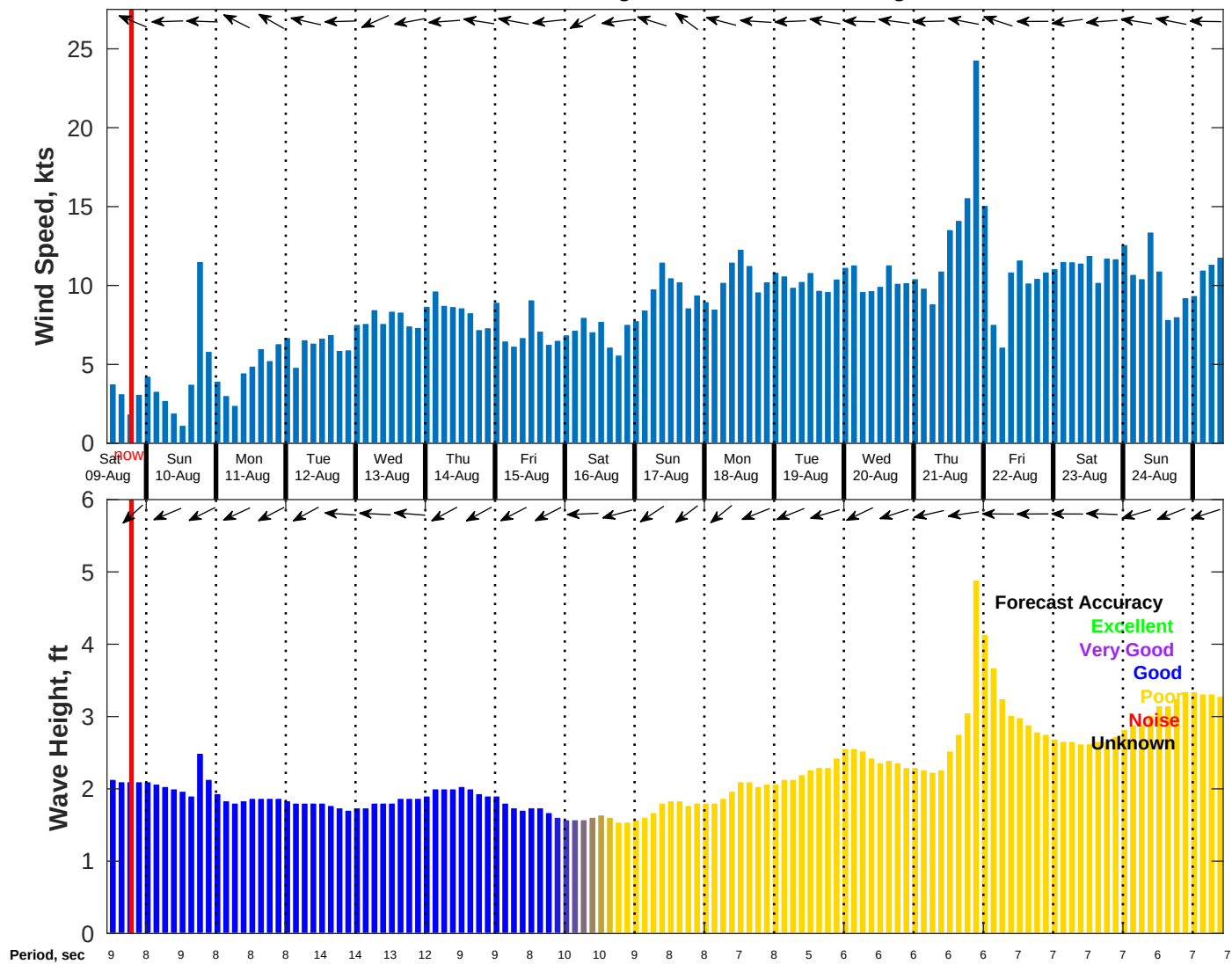
Wind & Wave Forecast for NDBC 52213 from 08-Aug-2025 11:00:00 to 24-Aug-2025 11:00:00
