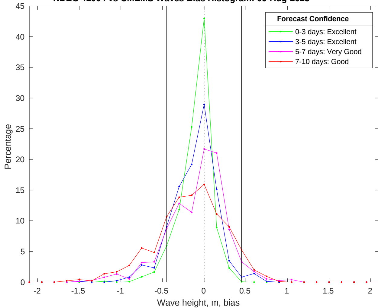
NDBC 41004 vs CMEMS Waves Bias Histogram: 09-Aug-2025
