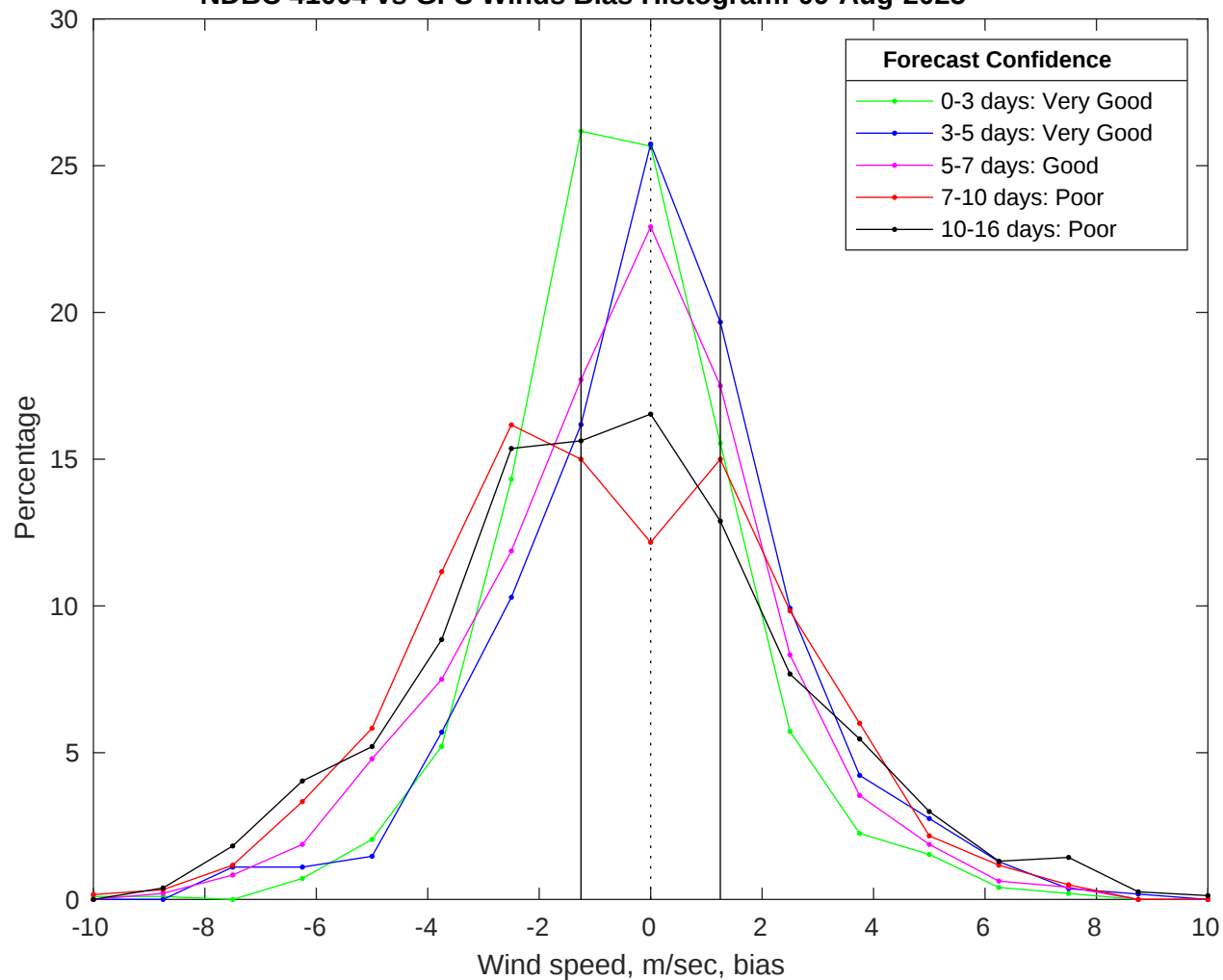
NDBC 41004 vs GFS Winds Bias Histogram: 09-Aug-2025
