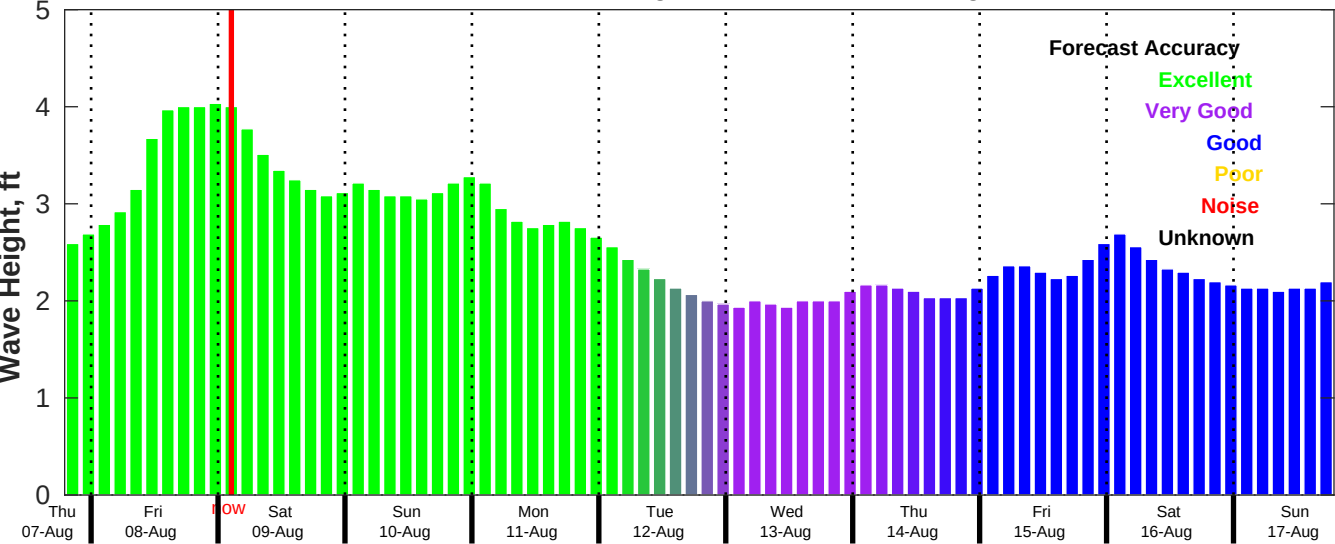
CMEMS Wave Forecast for NDBC 41004 from 07-Aug-2025 19:00:00 to 17-Aug-2025 19:00:00
