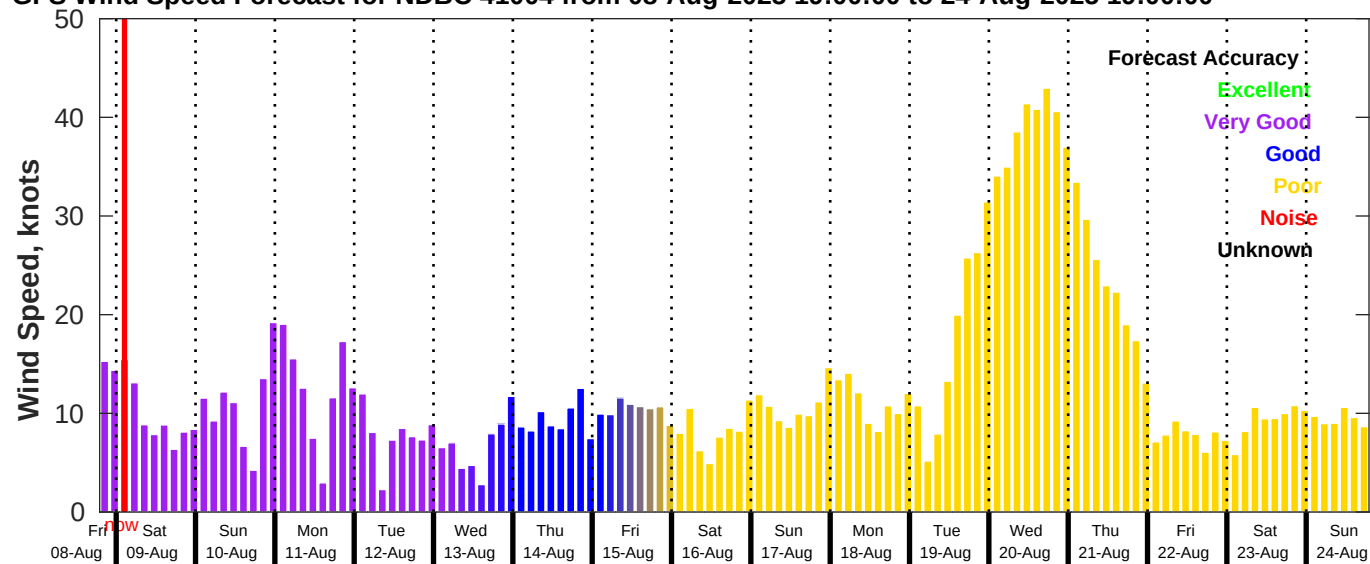
GFS Wind Speed Forecast for NDBC 41004 from 08-Aug-2025 19:00:00 to 24-Aug-2025 19:00:00
