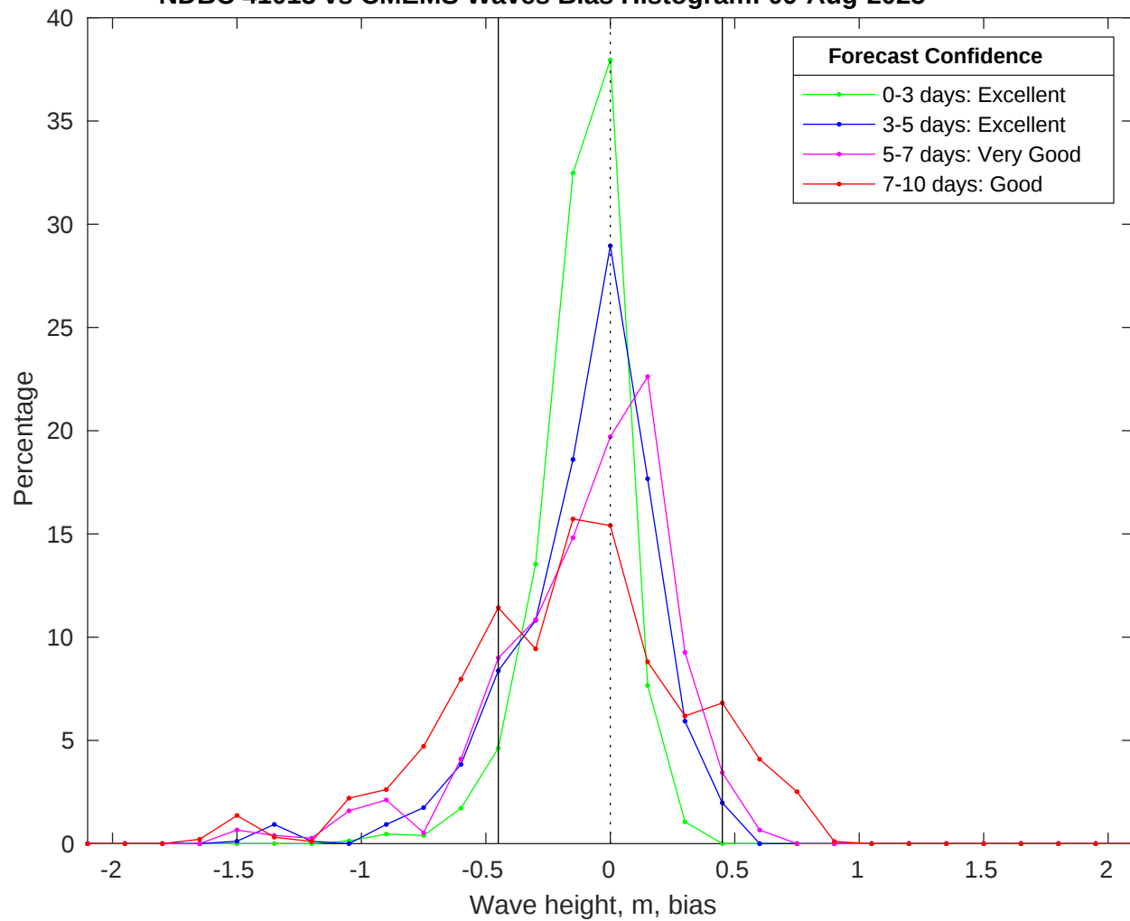
NDBC 41013 vs CMEMS Waves Bias Histogram: 09-Aug-2025
