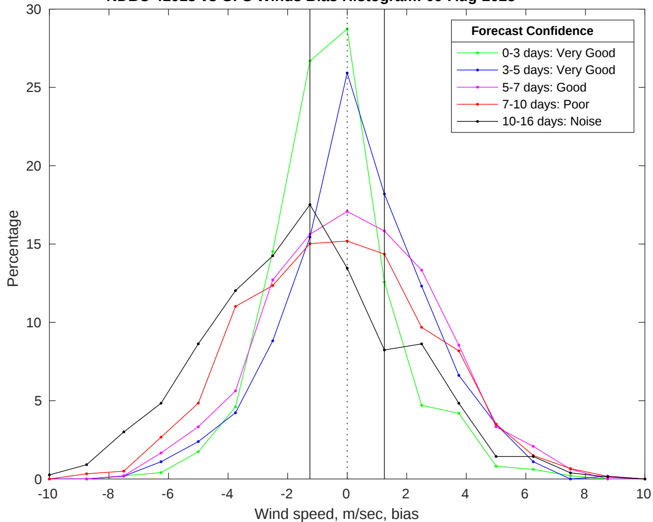
NDBC 41013 vs GFS Winds Bias Histogram: 09-Aug-2025
