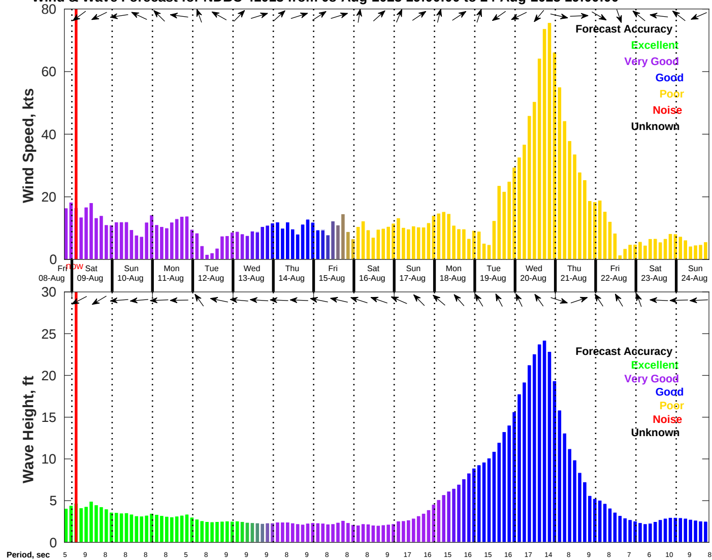
Wind & Wave Forecast for NDBC 41013 from 08-Aug-2025 19:00:00 to 24-Aug-2025 19:00:00
