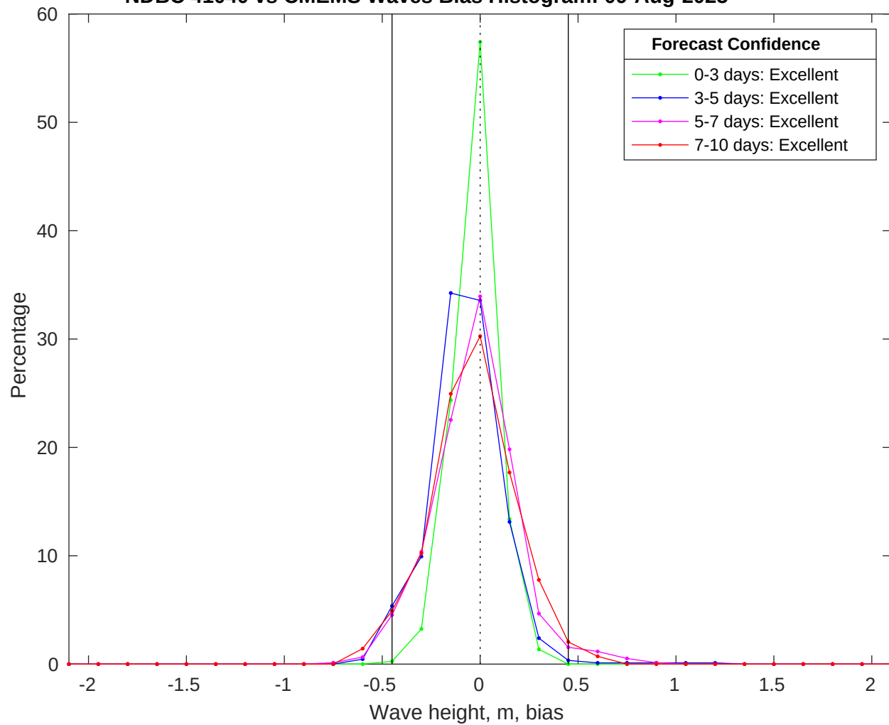
NDBC 41040 vs CMEMS Waves Bias Histogram: 09-Aug-2025
