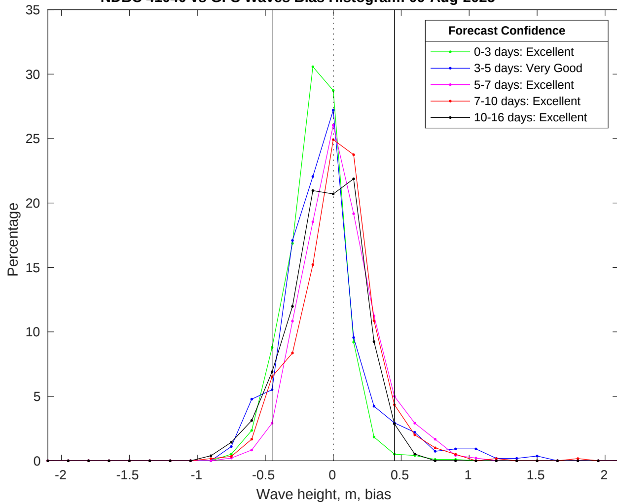
NDBC 41040 vs GFS Waves Bias Histogram: 09-Aug-2025
