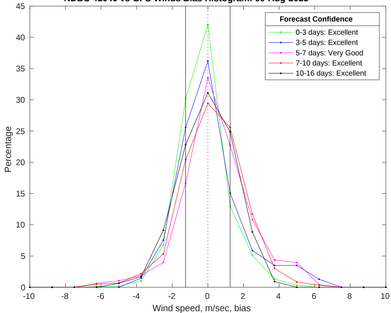
NDBC 41040 vs GFS Winds Bias Histogram: 09-Aug-2025
