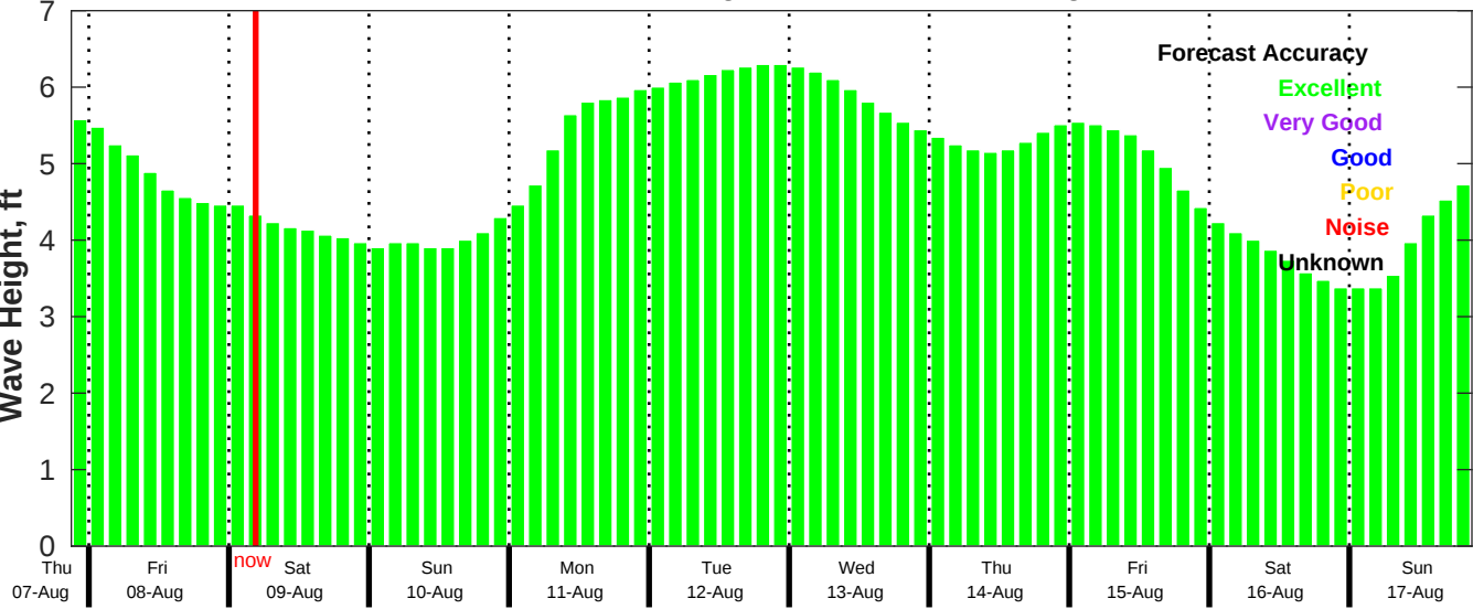
CMEMS Wave Forecast for NDBC 41040 from 07-Aug-2025 21:00:00 to 17-Aug-2025 21:00:00
