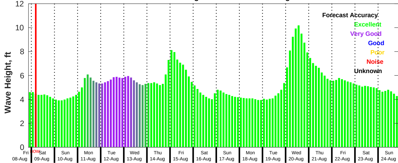
GFS Wave Forecast for NDBC 41040 from 08-Aug-2025 21:00:00 to 24-Aug-2025 21:00:00
