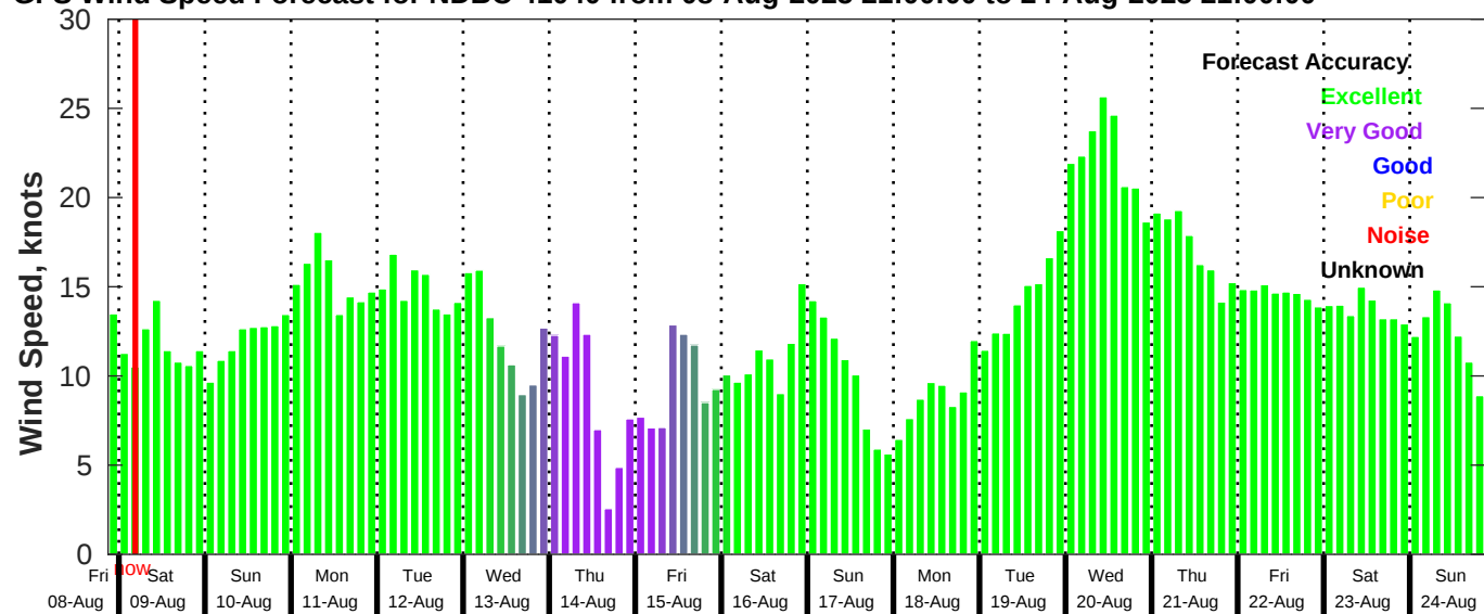
GFS Wind Speed Forecast for NDBC 41040 from 08-Aug-2025 21:00:00 to 24-Aug-2025 21:00:00
