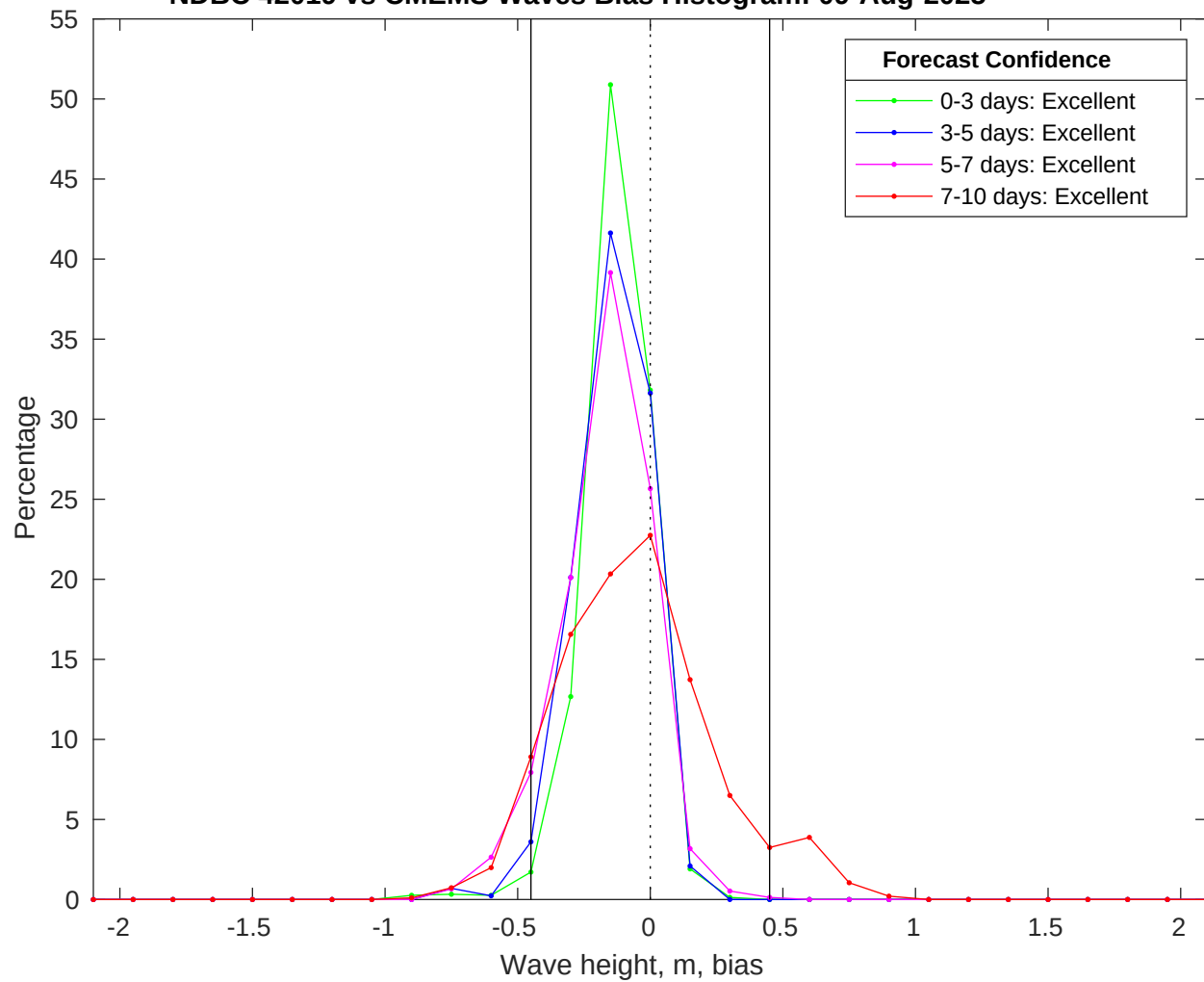
NDBC 42019 vs CMEMS Waves Bias Histogram: 09-Aug-2025
