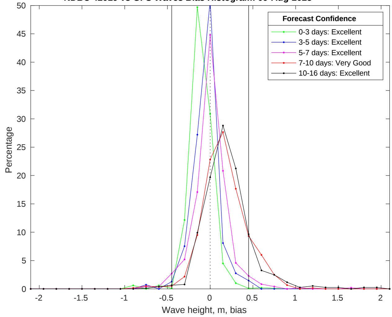
NDBC 42019 vs GFS Waves Bias Histogram: 09-Aug-2025
