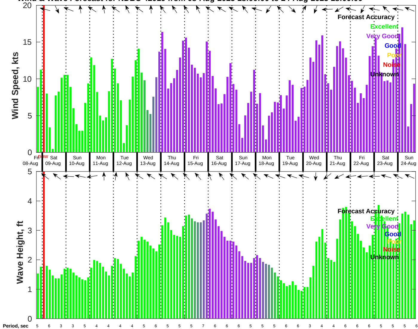
Wind & Wave Forecast for NDBC 42019 from 08-Aug-2025 18:00:00 to 24-Aug-2025 18:00:00
