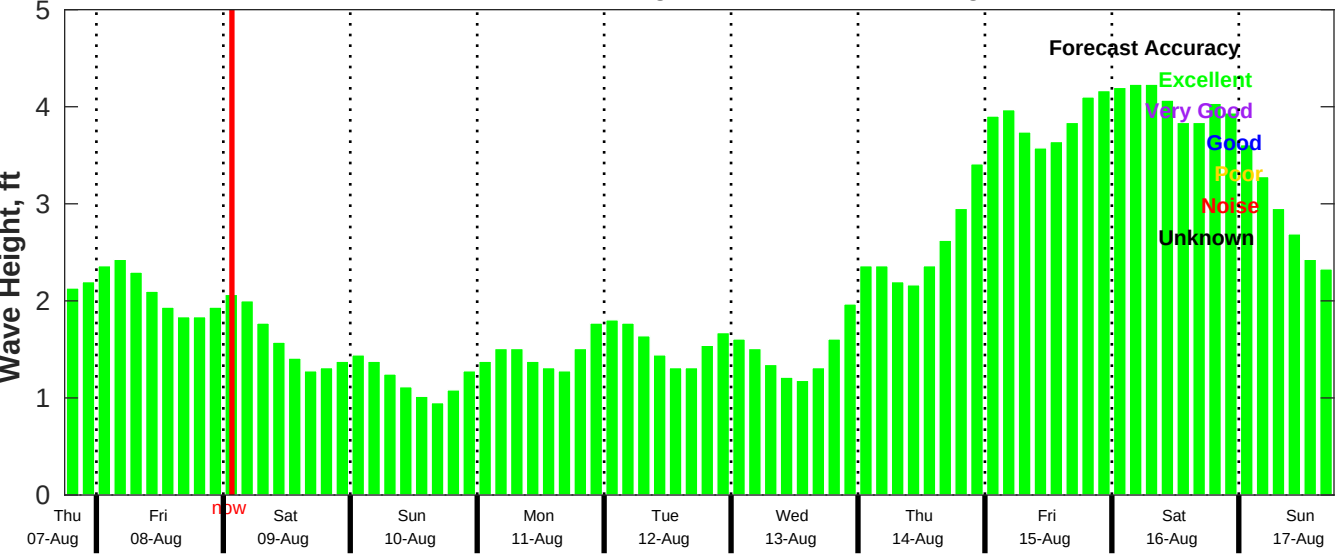
CMEMS Wave Forecast for NDBC 42020 from 07-Aug-2025 18:00:00 to 17-Aug-2025 18:00:00
