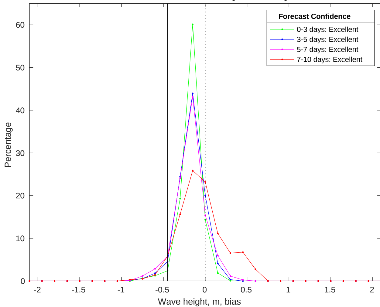
NDBC 42035 vs CMEMS Waves Bias Histogram: 09-Aug-2025
