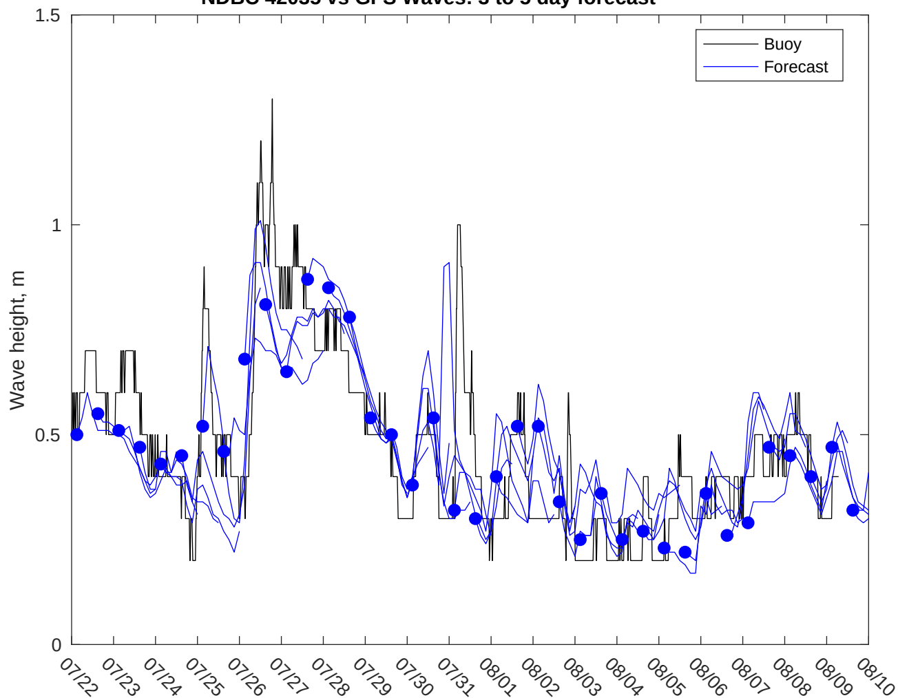
NDBC 42035 vs GFS Waves: 3 to 5 day forecast
