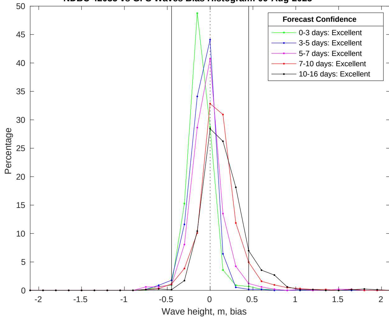
NDBC 42035 vs GFS Waves Bias Histogram: 09-Aug-2025
