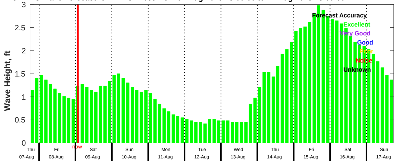
CMEMS Wave Forecast for NDBC 42035 from 07-Aug-2025 18:00:00 to 17-Aug-2025 18:00:00
