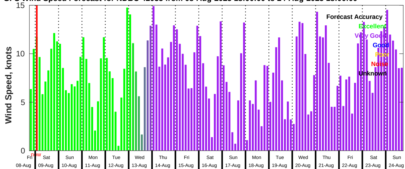
GFS Wind Speed Forecast for NDBC 42035 from 08-Aug-2025 18:00:00 to 24-Aug-2025 18:00:00
