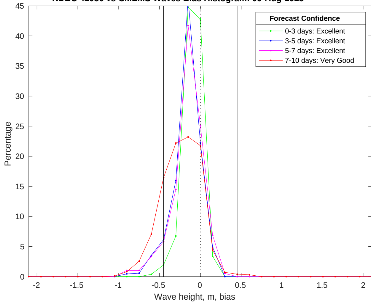
NDBC 42036 vs CMEMS Waves Bias Histogram: 09-Aug-2025
