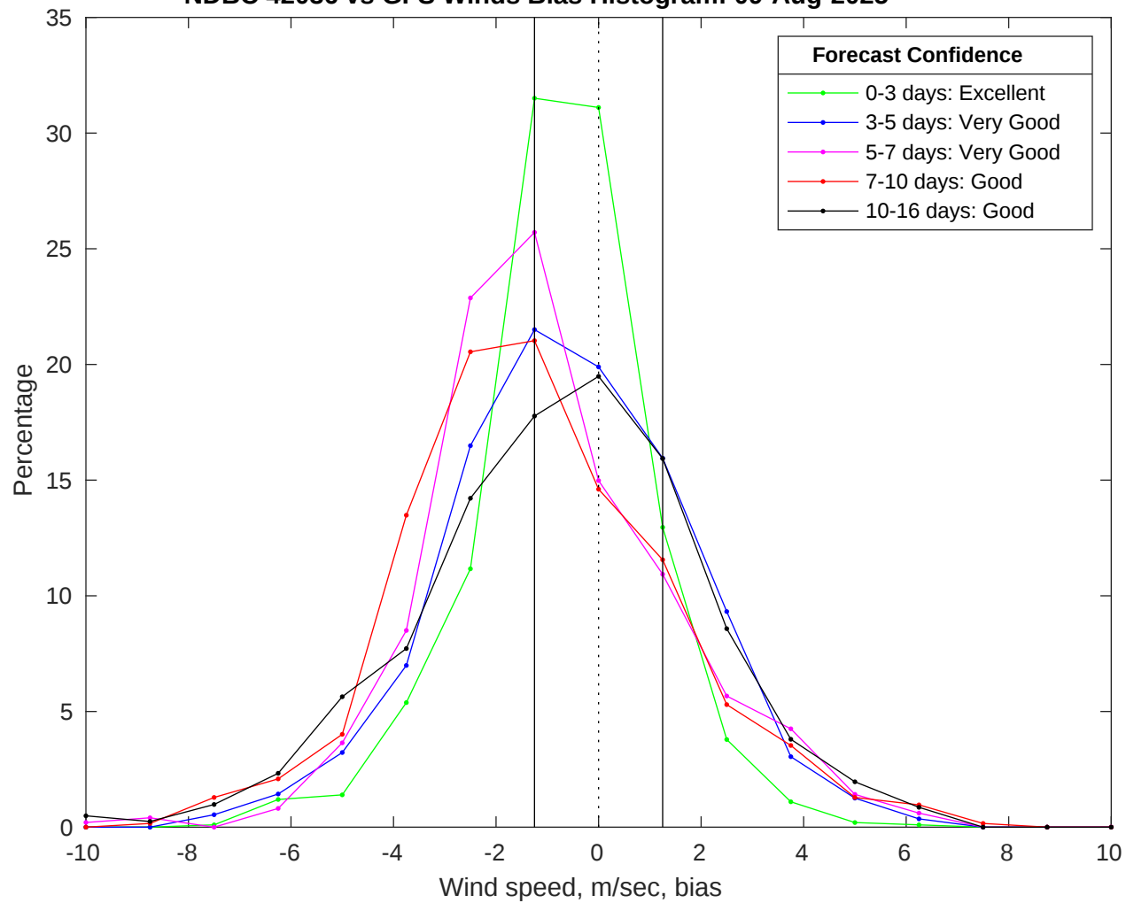
NDBC 42036 vs GFS Winds Bias Histogram: 09-Aug-2025
