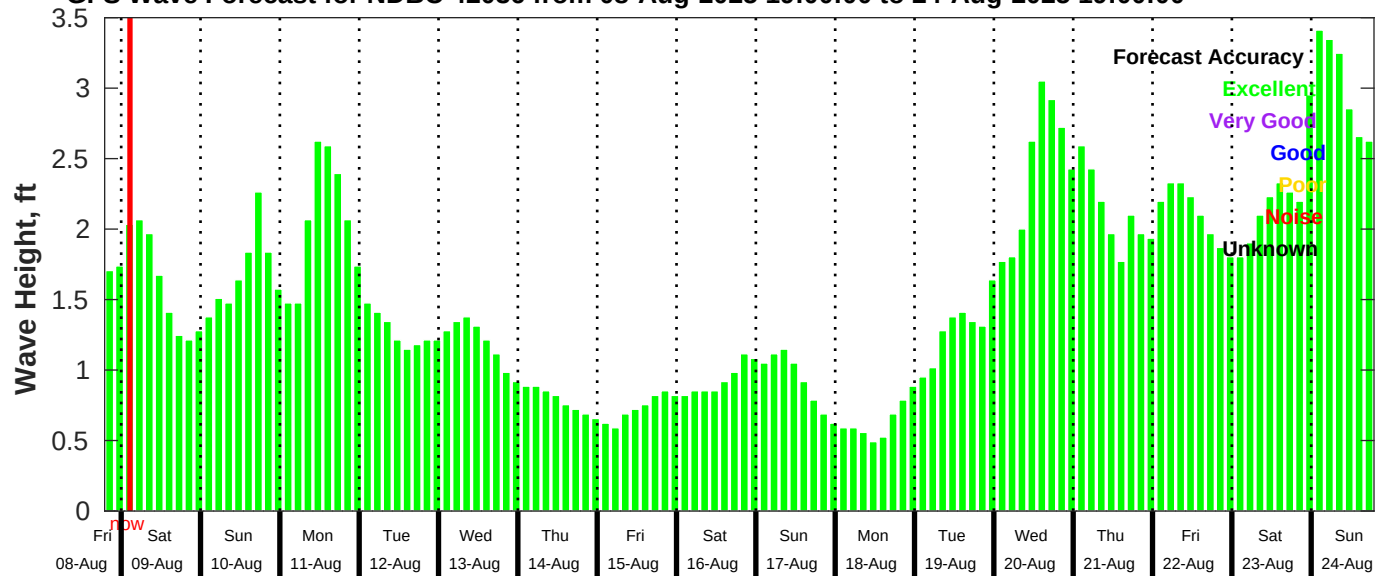
GFS Wave Forecast for NDBC 42036 from 08-Aug-2025 19:00:00 to 24-Aug-2025 19:00:00
